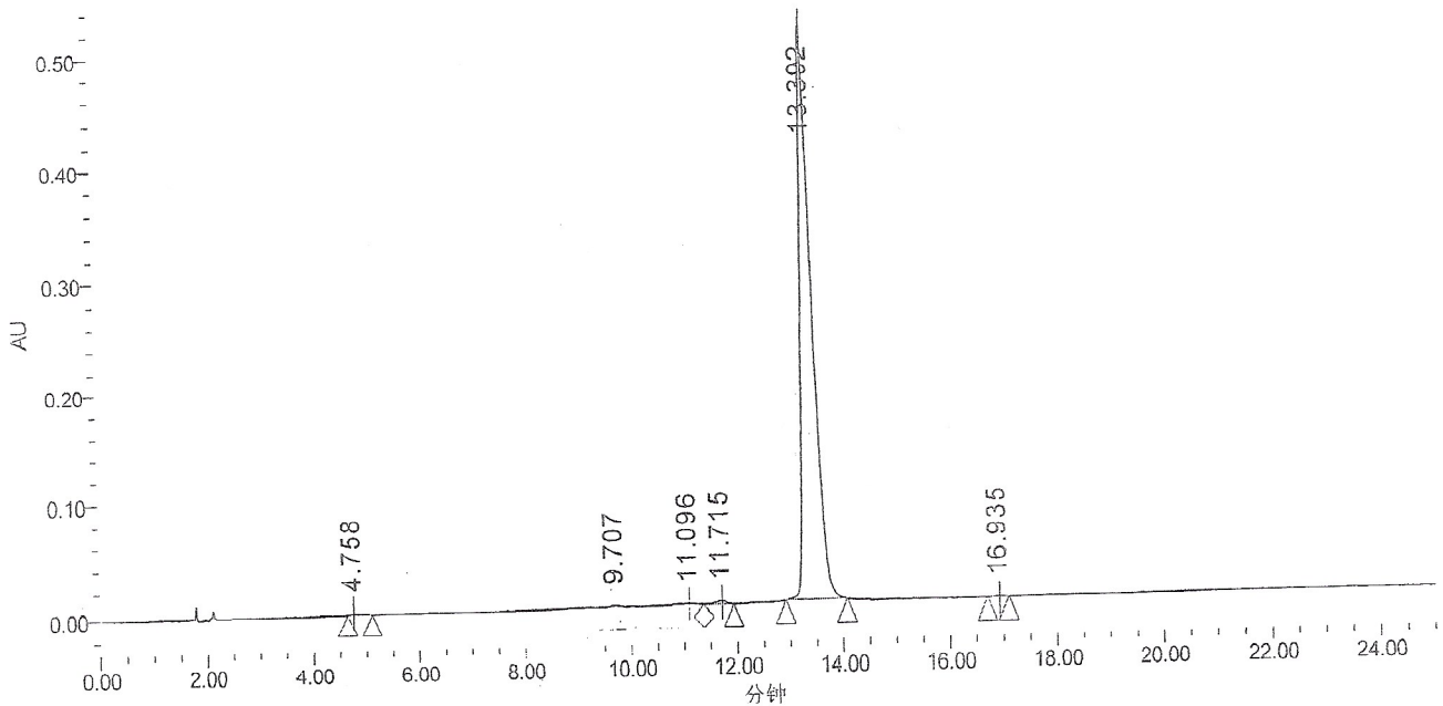
Auto-Scaled Chromatogram
